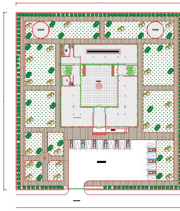
SITE PLAN
